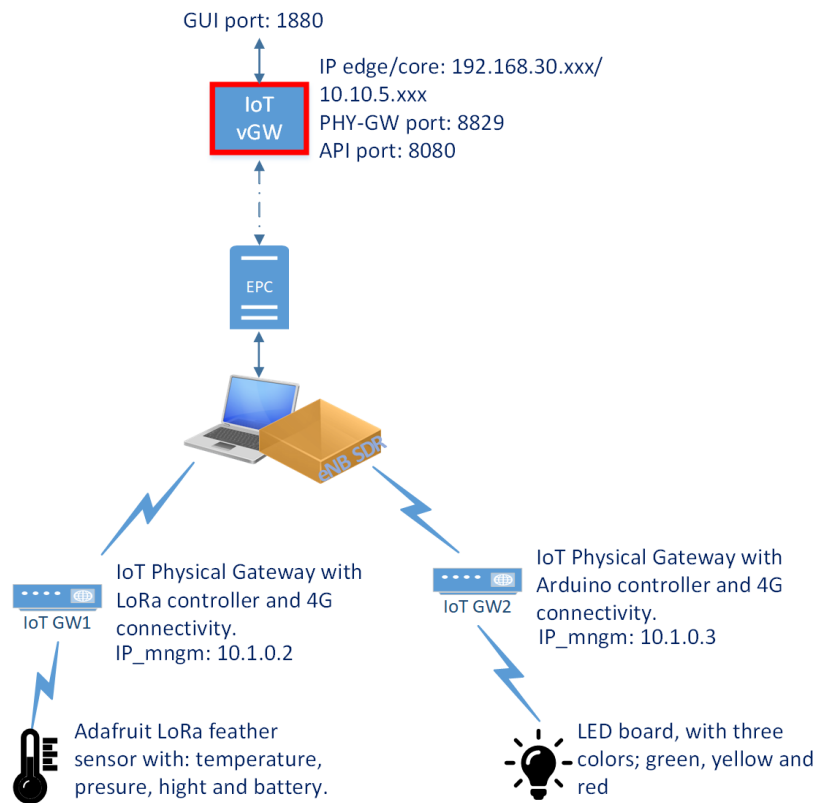
Figure 7-5: E2E Application latency measurement deployment and configuration.
