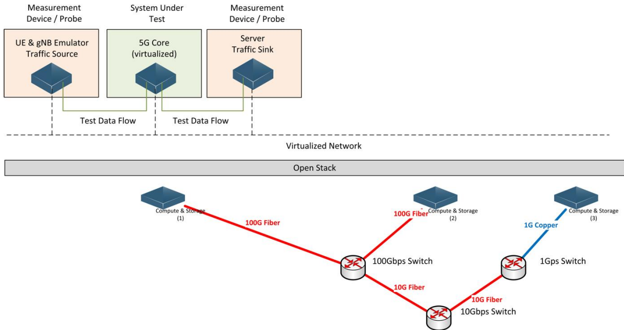
Figure 2-1: Example measurement system: clustered virtualized components.
