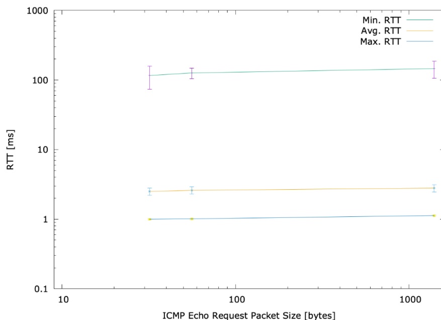
Figure 9-14 Round-Trip-Time observed for the MetroLinq 60 GHz backhaul
