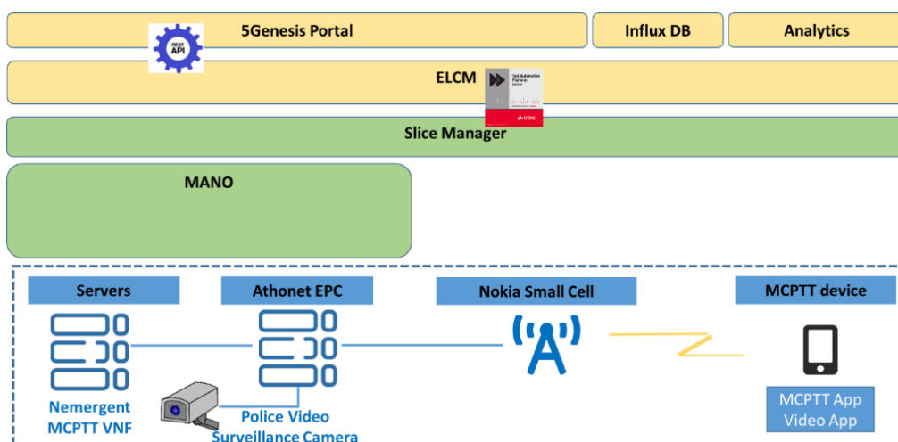
Figure 5-5 Malaga platform setup 2
