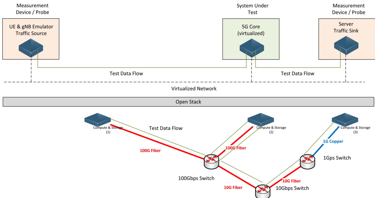
Figure 2-2 Example measurement system: distributed virtualized components.
