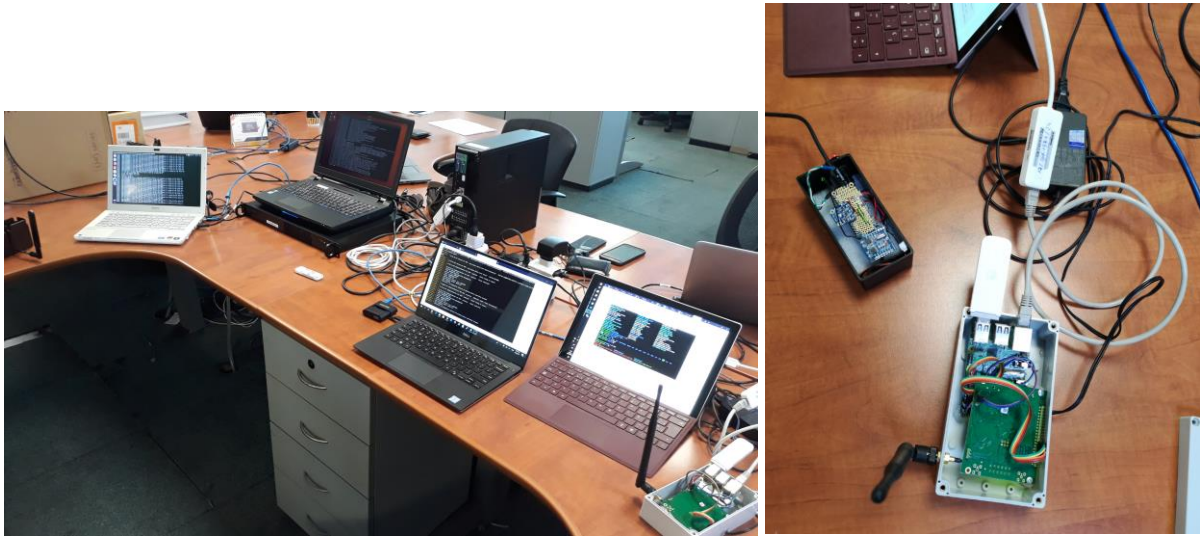
Figure 7-3 Limassol Platform experiments setup with Ues and IoT-oriented RANs
