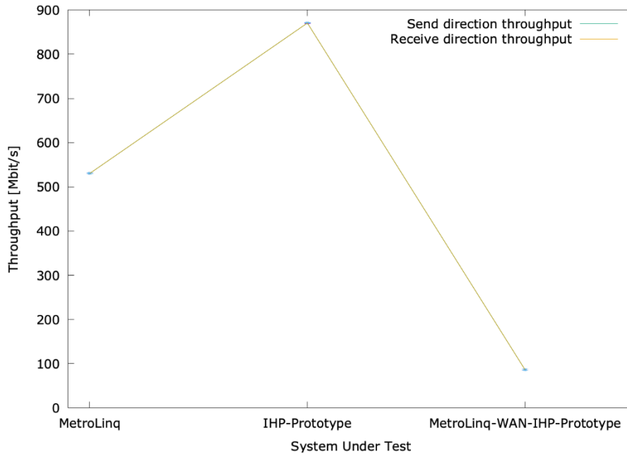
Figure 9-16 Throughput of the IHP 60 GHz backhaul system
