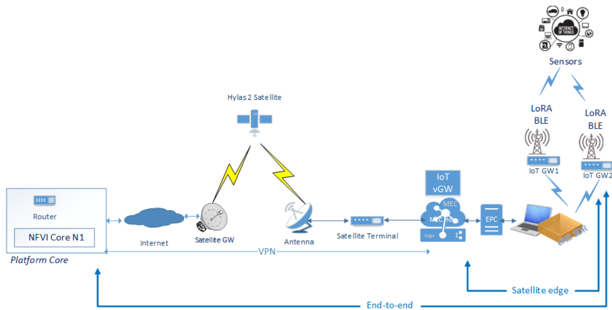
Figure 7-4. Measurement points in the Limassol platform
