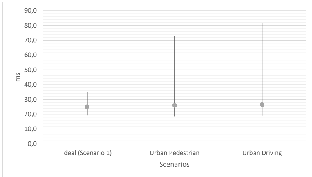
Figure 5-6 RTT results
