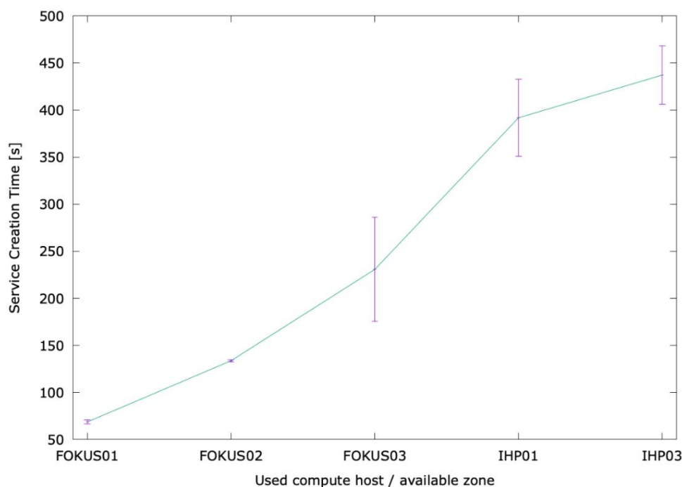
Figure 9-13 Service creation time calibration test – influence of VM placement
