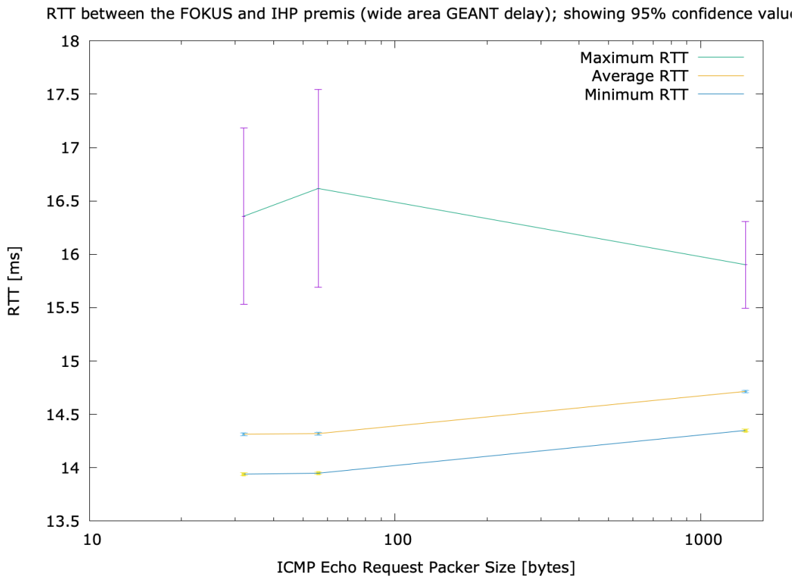
Figure 9-10 Round-Trip-Time between VNFs/VMs deployed in different availability interconnected via a wide-area, GEANT-based link
