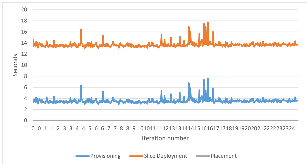
Figure 5-10 Raw results of the service creation time calibration test
