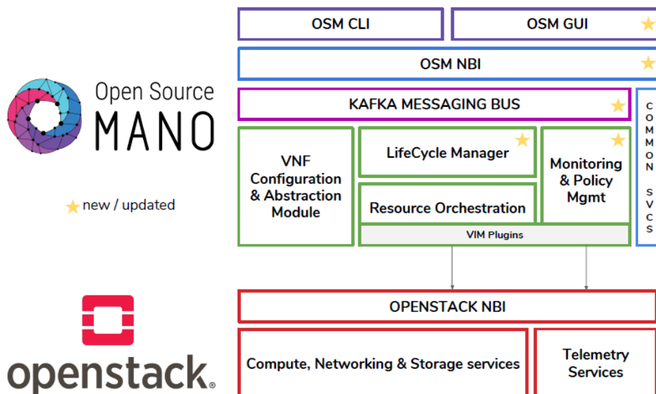
Figure 8-6: The architecture as adopted by the Surrey platform
