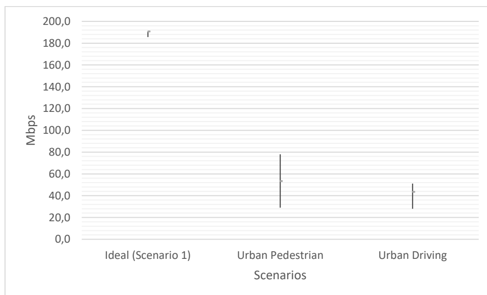
Figure 5-7 User data rate results
