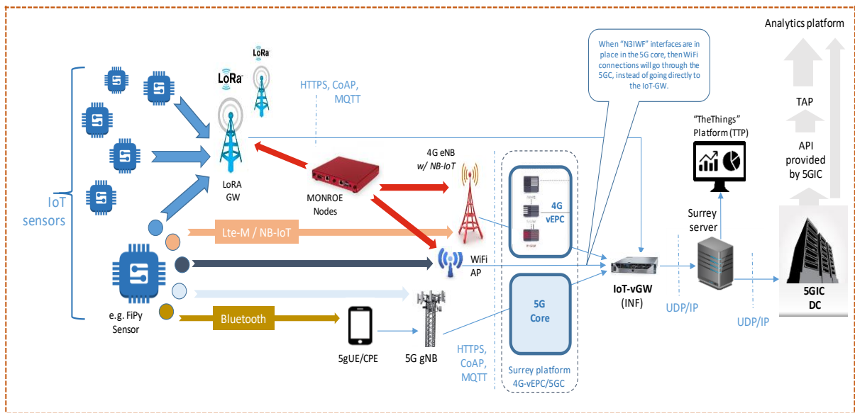
Figure 8-5: Network topology for the use case scenario at the 5GIC/ICS Site
