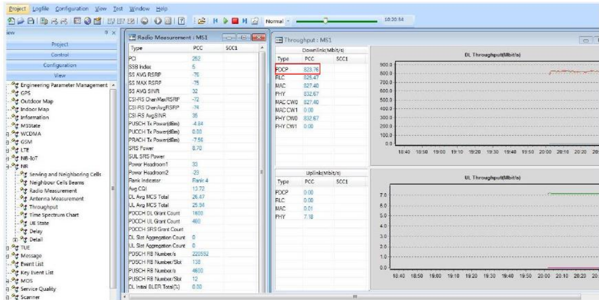
Figure 8-2 Results snapshot (BBU 26 NR cell 252) - Surrey Platform Phase I Trials, for UDP peak traffic.
