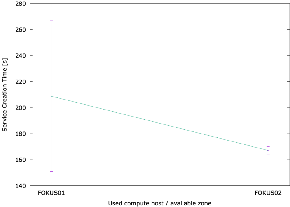
Figure 9-20 Service creation time of the Open5GCore Rel.3 packet core
