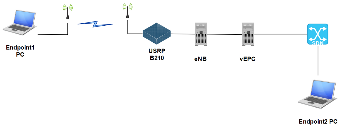
Figure 6-3 Laboratory configuration
