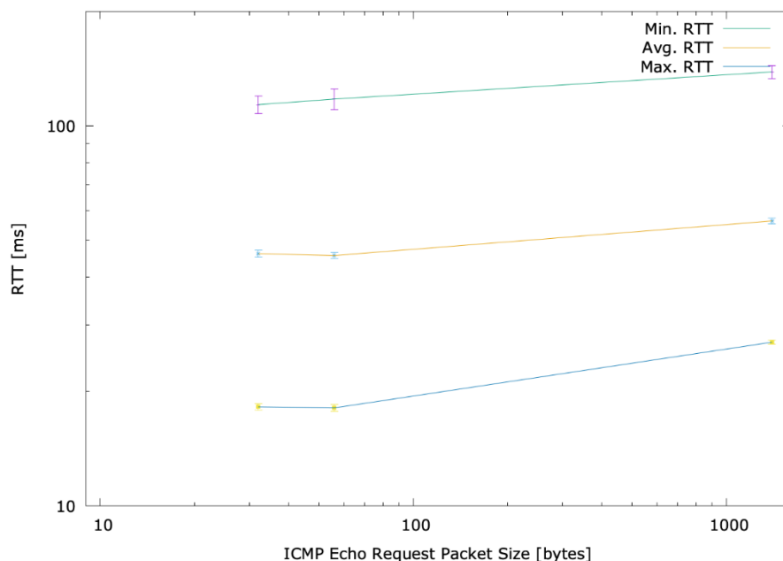
Figure 9-18 E2E network layer RTT evaluation of the Open5GCore Rel.3 packet core
