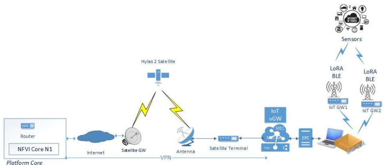
Figure 7-1. Actual topology of Limassol platform implemented for Phase 1 experimentation
