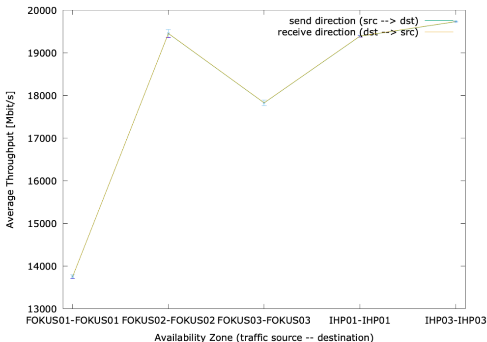
Figure 9-12 Average Throughput between VNFs/VMs deployed in the same availability zone
